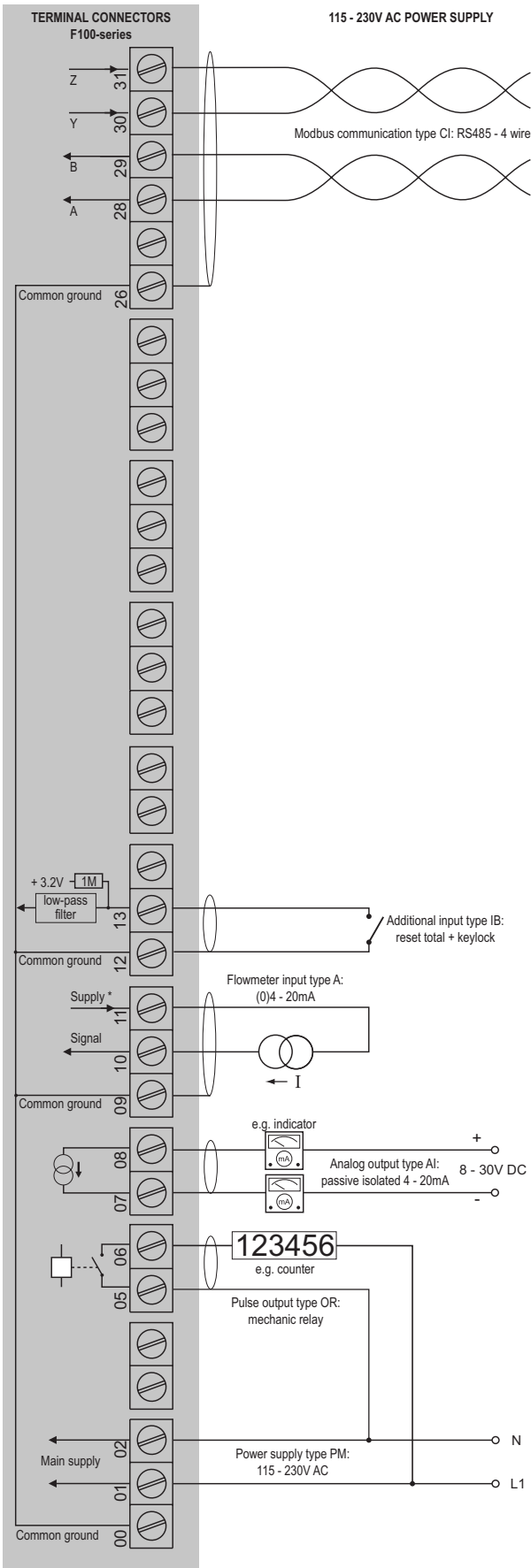
Configuration example F112-A-AI-CI-IB-OR-PM-XX-ZX
