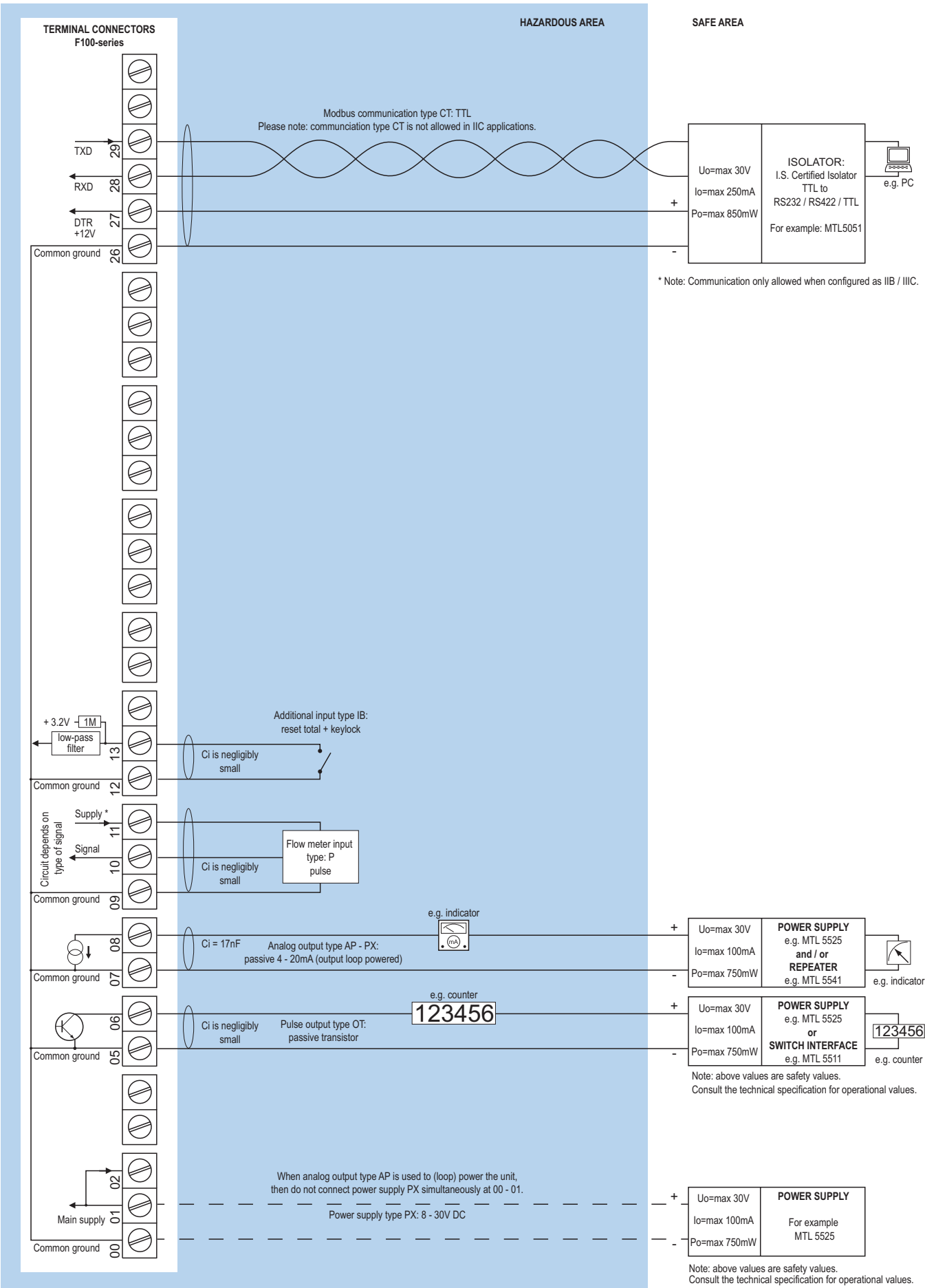
Configuration example IIB / IIIC and IIC - F112-P-AP-(CT)-IB-OT-(PX)-XI - Output loop powered
