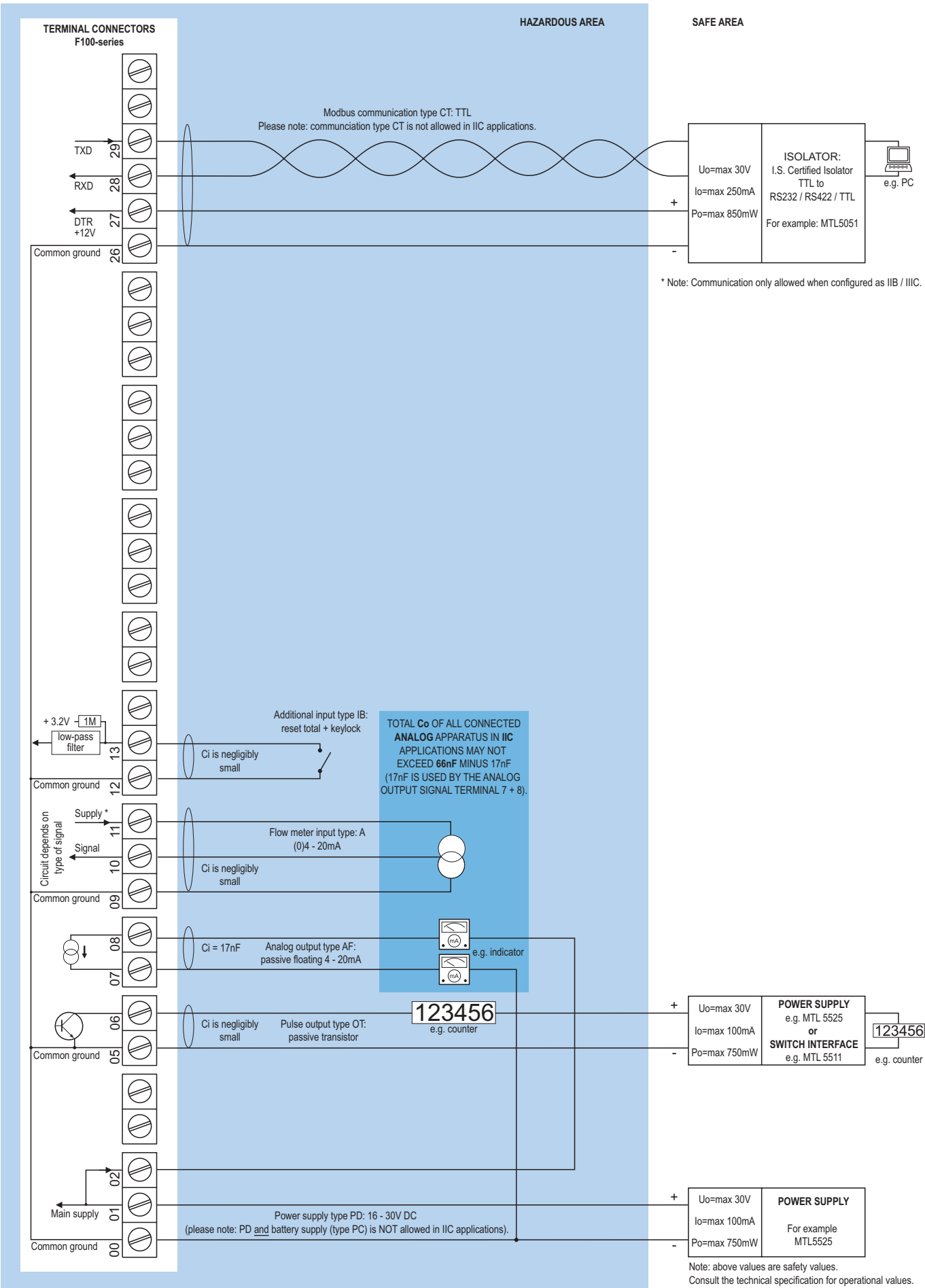
Configuration example IIB / IIIC and IIC - F112-A-AF-(CT)-IB-OT-PD-XI - Power requirement 16 - 30V DC
