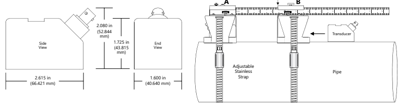
SE16A, SE16B, & SE16C Transducers & Mounting
